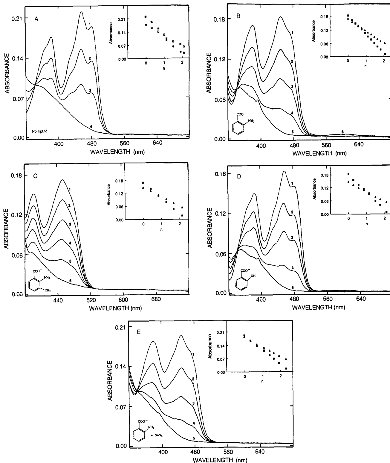
FIGURE 1: (A) Coulometric titration of anthranilate hydroxylase (18.5 \mu M enzyme) in 0.05 M potassium phosphate and 0.1 mM EDTA, pH 8.0, at 4 ^{\circ} C: (1) oxidized enzyme; (2) n = 0.69 ; (3) n = 1.5 ; (4) reduced enzyme. The inset shows the absorbance vs number of reducing equivalents added plotted for (■) 456 and (□) 383 nm. (B) Coulometric titration of anthranilate hydroxylase in the presence of anthranilate (15.1 \mu M enzyme) in 0.05 M potassium phosphate, 0.1 mM EDTA, and 0.6 mM anthranilate, pH 7.6, at 4 ^{\circ} C: (1) oxidized enzyme; (2) n = 0.57 ; (3) n = 1.11 ; (4) n = 1.64 ; (5) reduced enzyme, spectrum of reduced methyl viologen appears ( \lambda_{\max} , 603 and 395 nm). The inset shows the absorbance vs number of reducing equivalents added plotted for (■) 450 and (▲) 381 nm. (C) Coulometric titration of anthranilate hydroxylase in the presence of 3-methylantranilate (14.2 \mu M enzyme) in 0.05 M potassium phosphate, 0.1 mM EDTA, and 0.02 M 3-methylantranilate, pH 7.6, at 4 ^{\circ} C: (1) oxidized enzyme; (2) n = 0.42 ; (3) n = 0.83 ; (4) n = 1.27 ; (5) n = 1.66 ; (6) reduced enzyme. The inset shows the absorbance vs number of reducing equivalents added plotted for (■) 456 and (▲) 382 nm. (D) Coulometric titration of anthranilate hydroxylase in the presence of salicylate (15.1 \mu M enzyme) in 0.05 M potassium phosphate, 0.1 mM EDTA, and 1.2 mM sodium salicylate, pH 7.6, at 4 ^{\circ} C: (1) oxidized enzyme; (2) n = 0.57 ; (3) n = 1.15 ; (4) n = 1.74 ; (5) reduced enzyme, spectrum of reduced methyl viologen appears ( \lambda_{\max} , 603 and 395 nm). The inset shows the absorbance vs number of reducing equivalents added plotted for (■) 456 and (▲) 384 nm. (E) Coulometric titration of anthranilate hydroxylase in the presence of azide and anthranilate (16.5 \mu M enzyme) in 0.05 M potassium phosphate, 0.1 mM EDTA, 0.1 M sodium azide, and 0.6 mM anthranilate, pH 7.6, at 4 ^{\circ} C: (1) oxidized enzyme; (2) n = 0.69 ; (3) n = 1.39 ; (4) n = 1.93 ; (5) reduced enzyme. The inset shows the absorbance vs number of reducing equivalents added plotted for (■) 449 and (▲) 380 nm.
