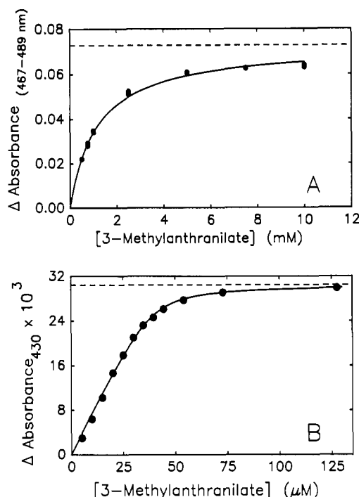
FIGURE 3: Titration of anthranilate hydroxylase with 3-methylantranilate at 3^\circ\text{C} as monitored by spectral perturbations. (A) Titration of oxidized enzyme ( 10.6 \mu\text{M} FAD) with 3-methylantranilate. This experiment was performed by mixing enzyme with ligand in a scanning stopped-flow spectrometer and recording the final spectra after the slow absorbance change ceased. Difference spectra were calculated for two separate shots. Filled circles ( \bullet ) are the data points, and the solid line ( — ) is the calculated (Duggleby, 1981) best fit with K_d = 1.13 \text{ mM} . \Delta A_{\text{max}} = 0.73 ( --- ). (B) Titration of reduced enzyme ( 39 \mu\text{M} ) with 3-methylantranilate. The enzyme, under an atmosphere of nitrogen, was reduced with an excess of sodium dithionite, and then aliquots of a solution of 3-methylantranilate were added anaerobically. Spectra were recorded vs buffer. The data points ( \bullet ) are plotted along with the calculated best fit ( — ), K_d = 1.65 \mu\text{M} ; the dashed line is the calculated \Delta A_{\text{max}} . The first two data points were not used in the fit.
